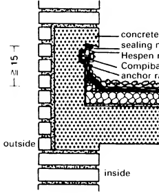
11 Wall connection: flanged connection with anchorage and Hespren rail
